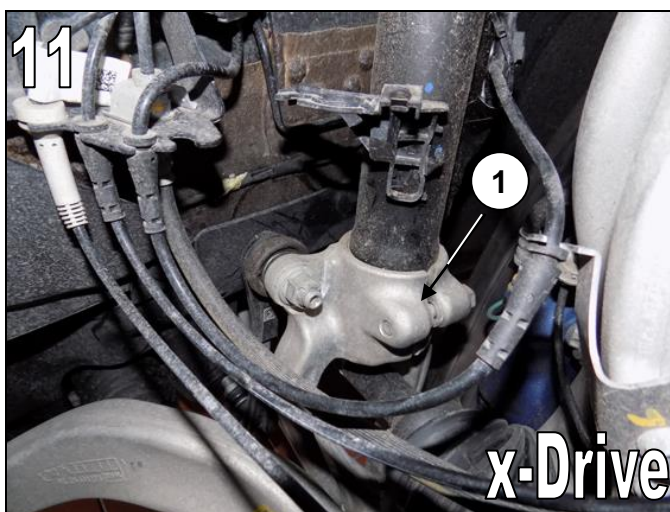
Fig. 11 x-Drive Spread swivel bearing / wheel carrier (1) using special tool 31 2 230 and pull down off spring strut.
